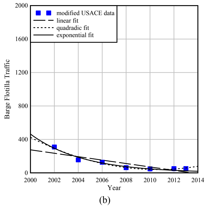
Figure E.8 Curve fits used to produce estimates of barge flotilla traffic for Dupont Bridge: (a) inbound direction; (b) outbound direction
