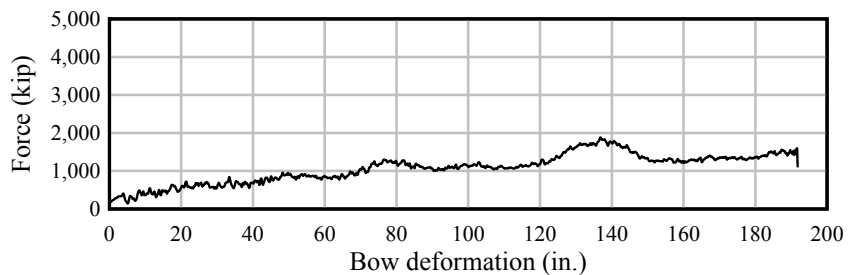
Figure D.32 Barge bow force-deformation data. 18-ft flat-faced pier surface at 45°
