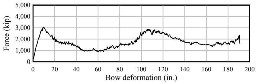
Figure D.47 Barge bow force-deformation data. 35-ft flat-faced pier surface at 1.5°
