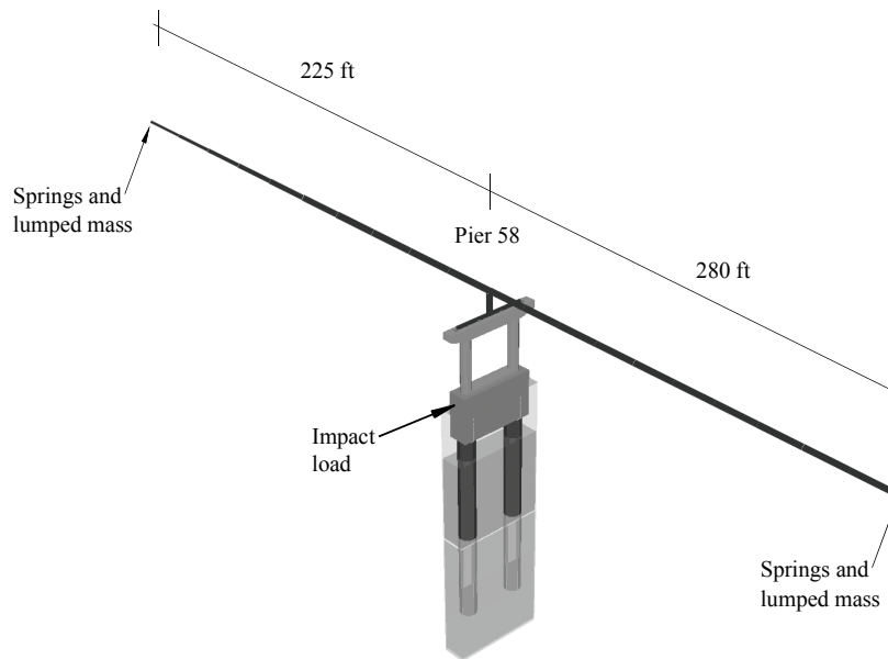
Figure 4.1 SR 20 at Blountstown, Pier 58 OPTS (BLT-CHA) model
