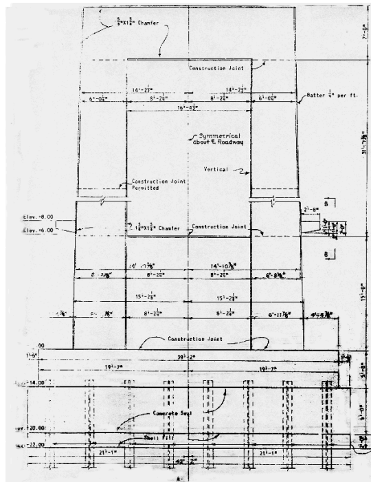
Figure 10-4 Original Construction Drawings for Pier-1
